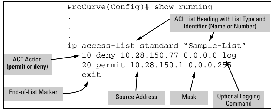
Figure 9-7. Example of a Displayed Standard ACL Configuration with Two ACEs
